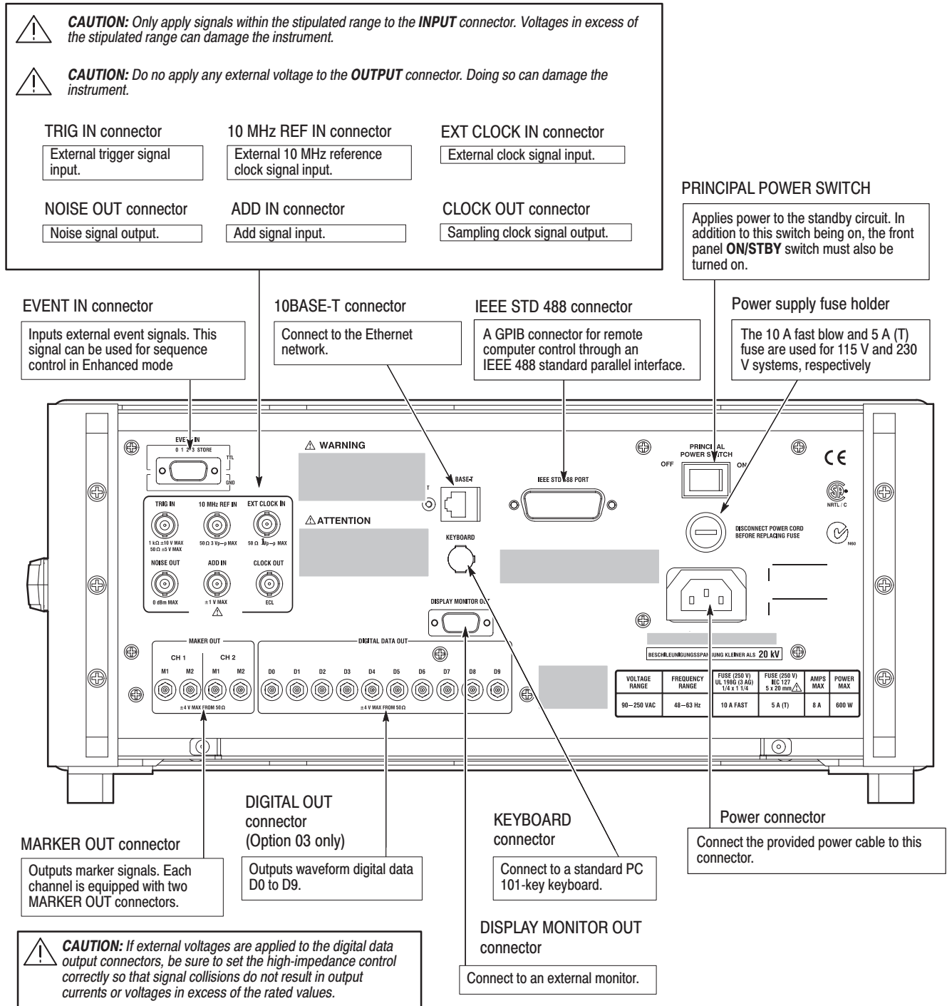
Figure 2-4: Rear panel map
